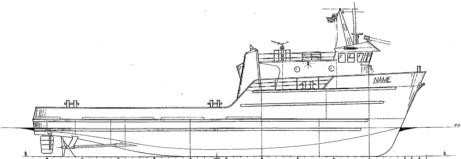
OUTBOARD PROFILE
