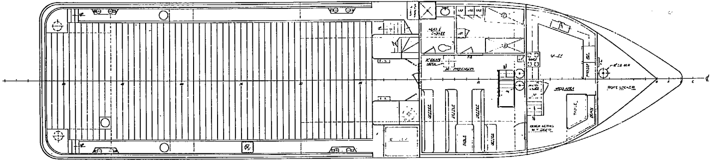
MAIN DECK
