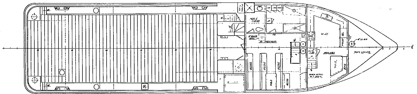
MAIN DECK
