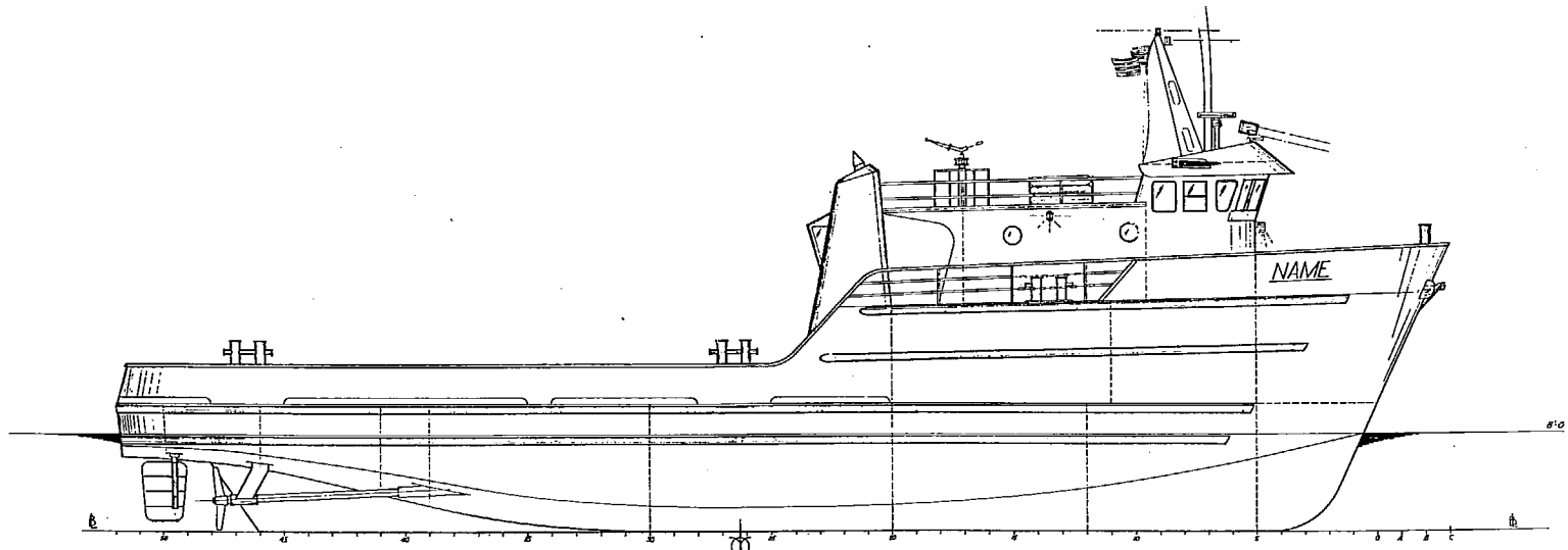
OUTBOARD PROFILE
